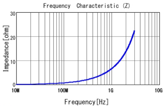
■ LQG15HS1N1S02 |Z|
