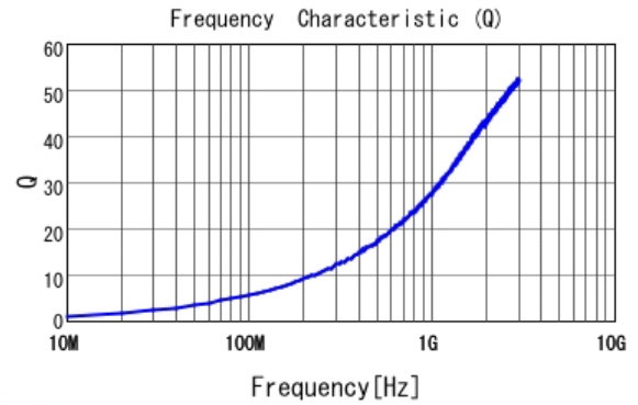
■ LQG15HS1N1S02 Q
