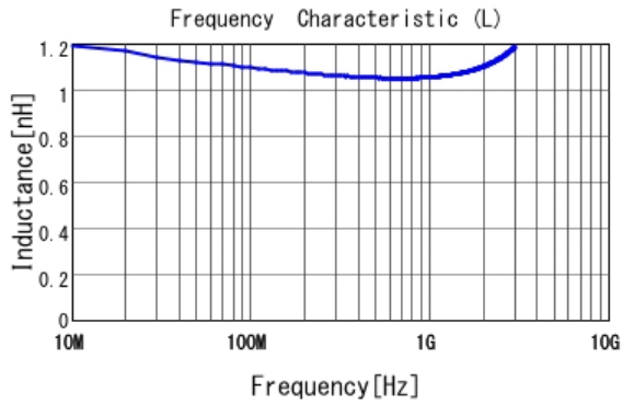
■ LQG15HS1N1S02 L
