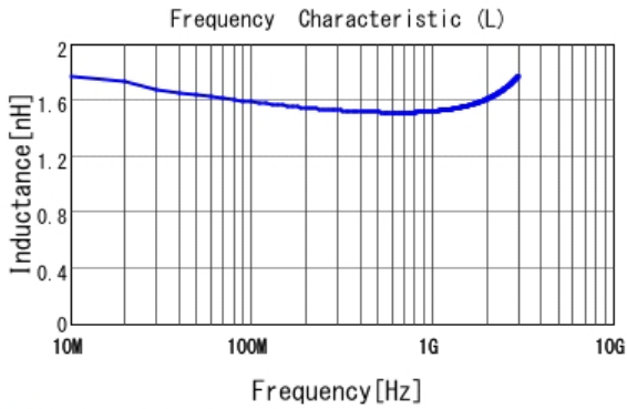
■ LQG15HS1N6S02 L
