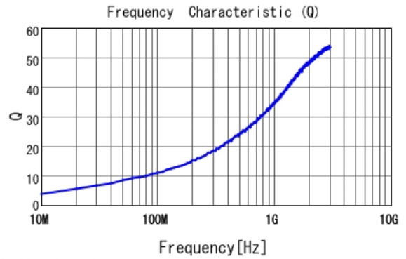
■ LQG15HS1N6S02 Q
