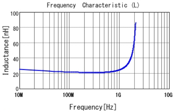
■ LQG15HS22NJ02 L
