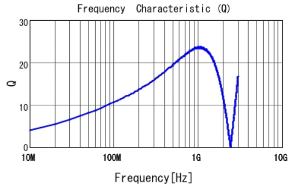
■ LQG15HS22NJ02 Q
