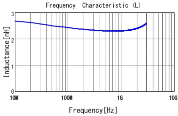
■ LQG15HS2N4S02 L
