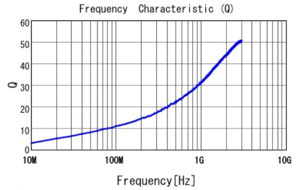
■ LQG15HS2N4S02 Q
