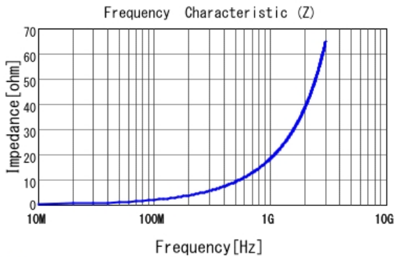
■ LQG15HS3N0S02 |Z|
