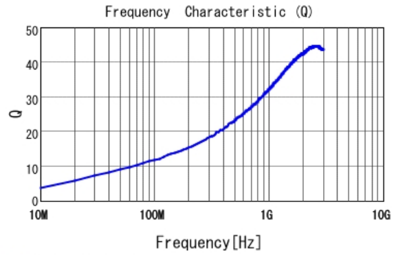
■ LQG15HS3N3S02 Q
