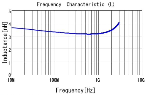
■ LQG15HS3N3S02 L
