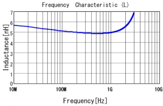
■ LQG15HS5N1S02 L
