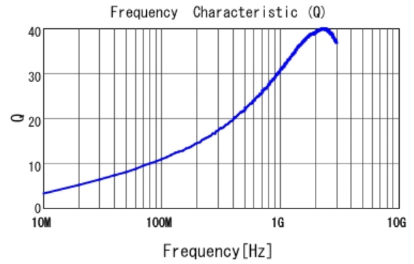
■ LQG15HS5N1S02 Q
