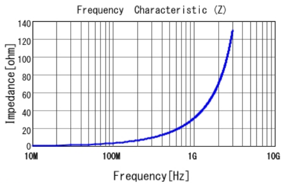
■ LQG15HS5N1S02 |Z|
