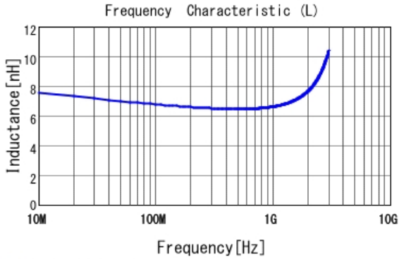
■ LQG15HS6N8J02 L
