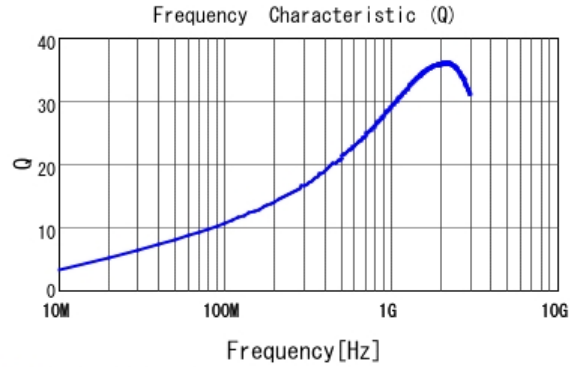
■ LQG15HS6N8J02 Q
