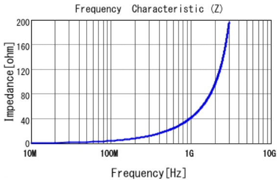
■ LQG15HS6N8J02 |Z|
