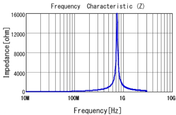
■ LQG15HSR18J02 |Z|
