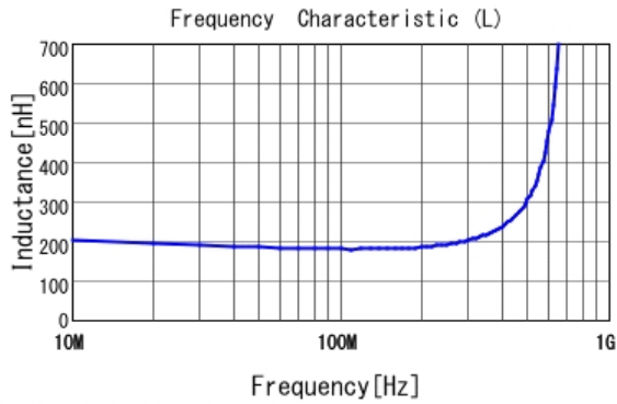
■ LQG15HSR18J02 L
