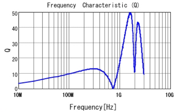
■ LQG15HSR18J02 Q
