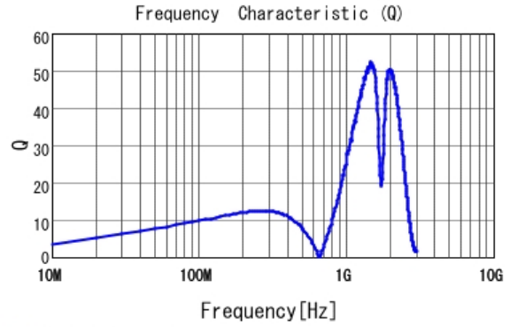
■ LQG15HSR22J02 Q
