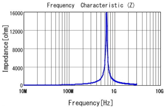
■ LQG15HSR22J02 |Z|
