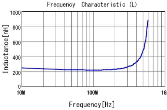
■ LQG15HSR22J02 L
