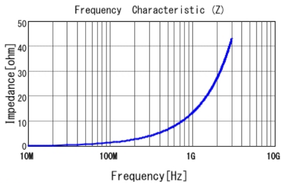
■ LQG18HN2N2S00 |Z|
