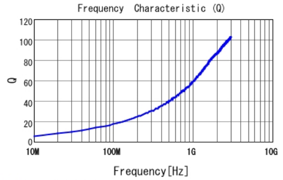
■ LQG18HN2N2S00 Q
