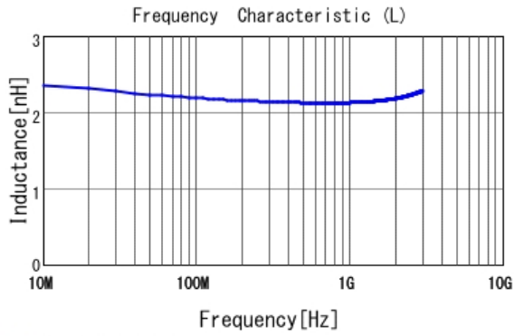
■ LQG18HN2N2S00 L
