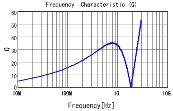
■ LQG18HN33NJ00 Q
