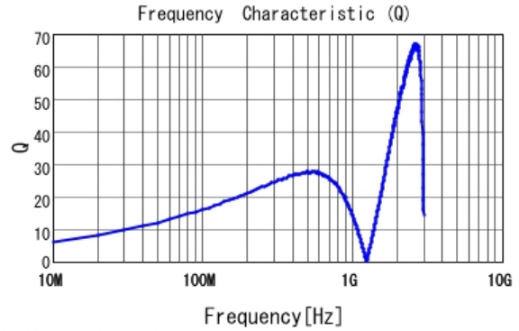
■ LQG18HN68NJ00 Q
