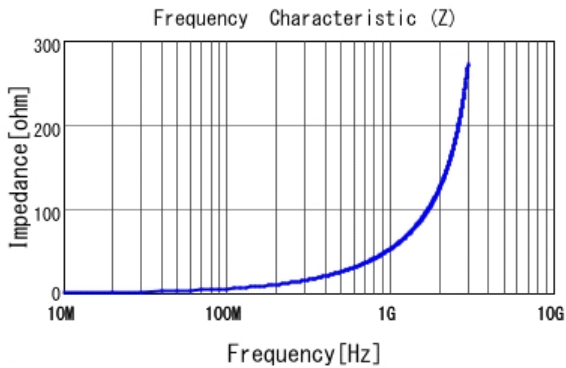
■ LQG18HN8N2J00 |Z|
