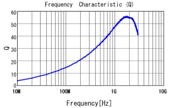
■ LQG18HN8N2J00 Q
