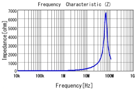
■ LQH2HPN4R7MJR |Z|
