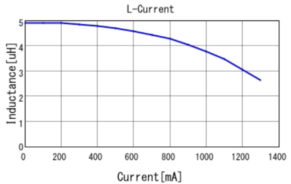
■ LQH2HPN4R7MJR L-Current 20degC
