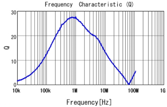
■ LQH2HPN4R7MJR Q
