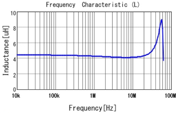
■ LQH2HPN4R7MJR L
