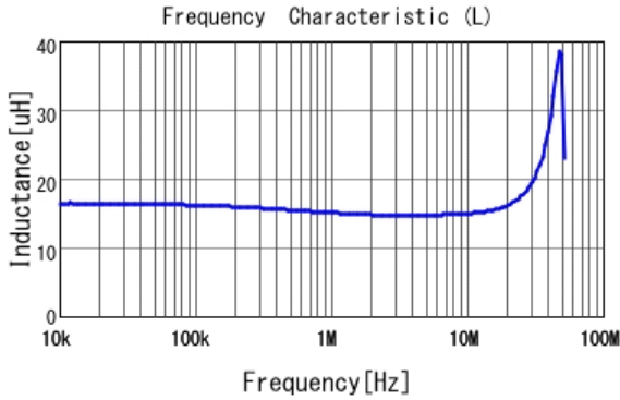
■ LQH2MCN150K02 L
