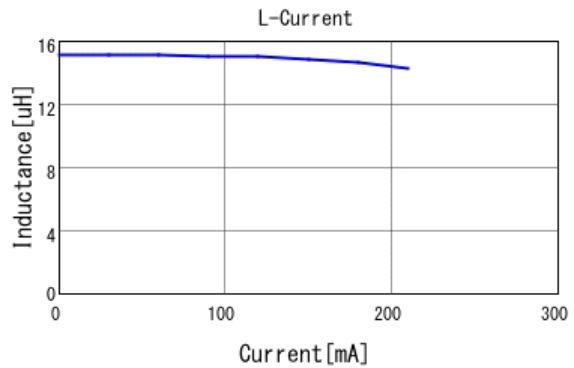
■ LQH2MCN150K02 L-Current 20degC
