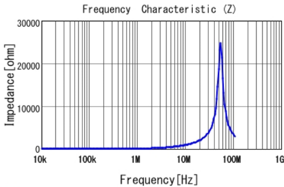
■ LQH2MCN150K02 |Z|
