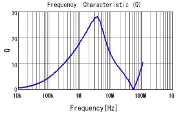
■ LQH2MCN150K02 Q
