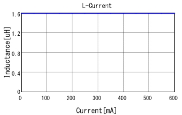
LQH2MCN1R5M02 L-Current 20degC
