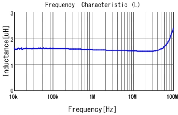
LQH2MCN1R5M02 L
