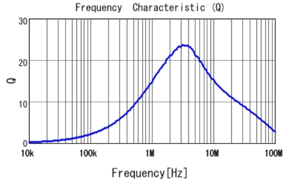
LQH2MCN1R5M02 Q
