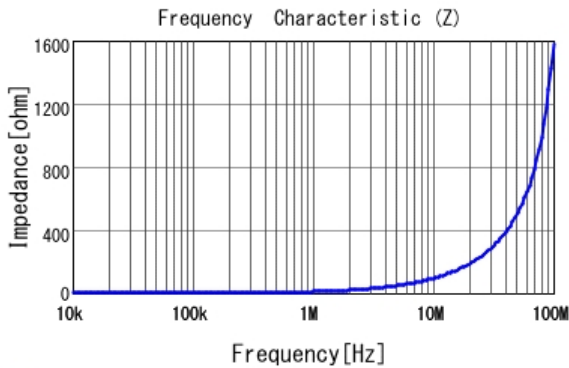
LQH2MCN1R5M02 |Z|
