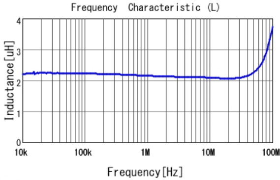
■ LQH2MCN2R2M02 L
