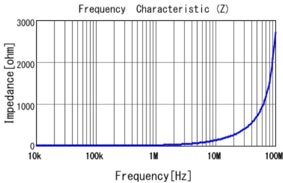
■ LQH2MCN2R2M02 |Z|
