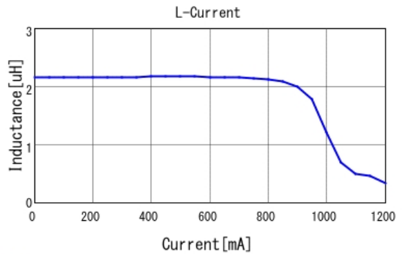
■ LQH2MCN2R2M02 L-Current 20degC
