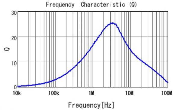
■ LQH2MCN2R2M02 Q
