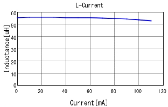
■ LQH2MCN560K02 L-Current 20degC
