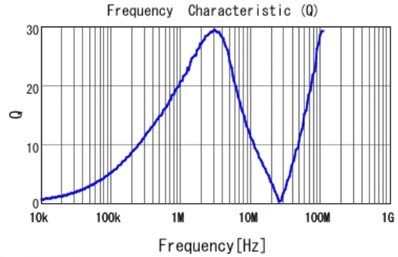
■ LQH2MCN560K02 Q
