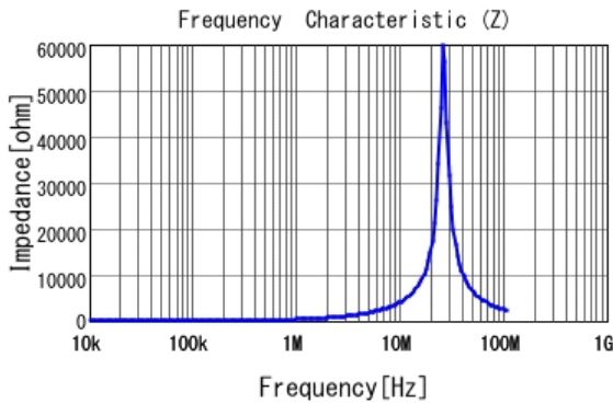
■ LQH2MCN560K02 |Z|
