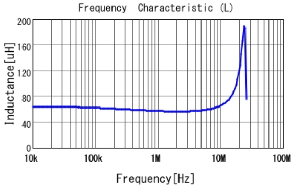
■ LQH2MCN560K02 L
