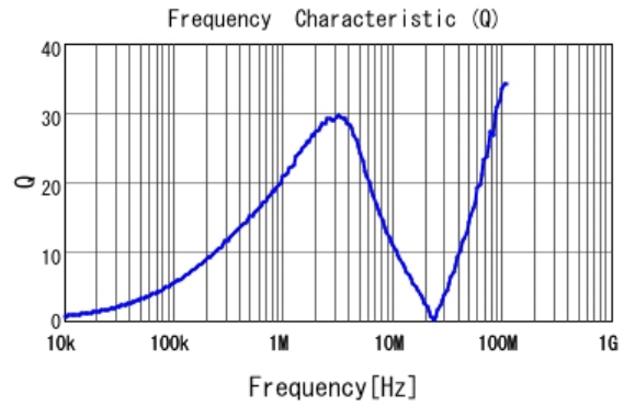
■ LQH2MCN680K02 Q
