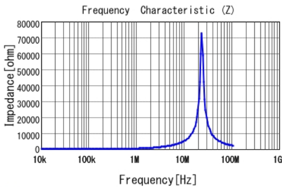
■ LQH2MCN680K02 |Z|
