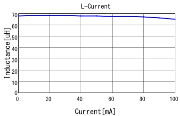
■ LQH2MCN680K02 L-Current 20degC
