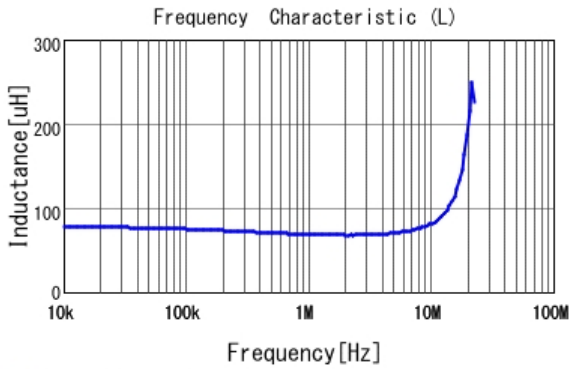
■ LQH2MCN680K02 L
