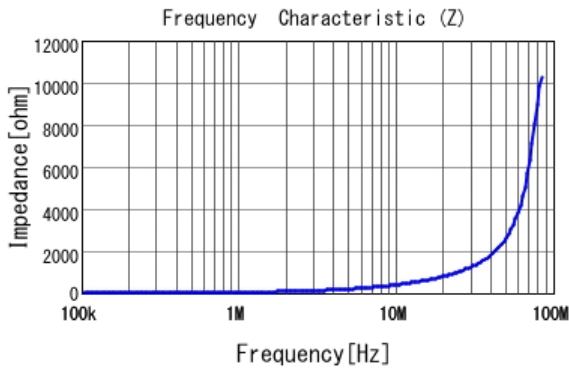
LQH2MCN6R8M52 |Z|
