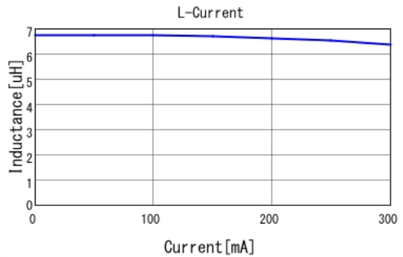
LQH2MCN6R8M52 L-Current 20degC
