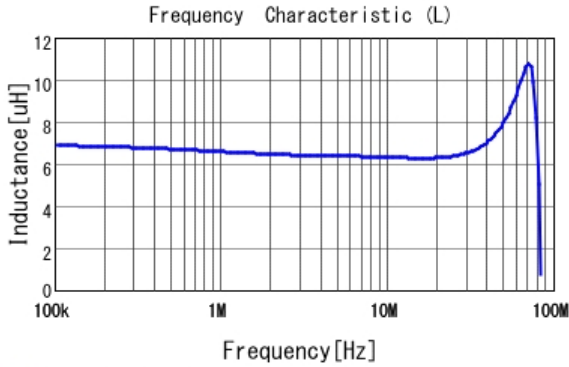
LQH2MCN6R8M52 L
