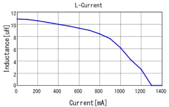
■ LQH32PB100MN0 L-Current 20degC
