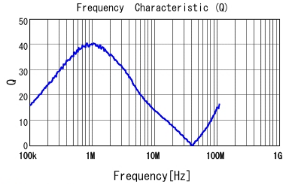
■ LQH32PB100MN0 Q
