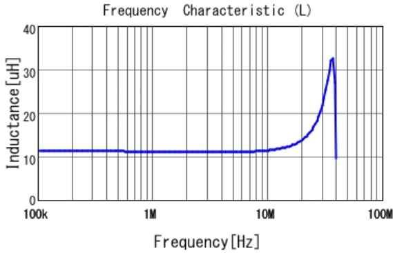
■ LQH32PB100MN0 L
