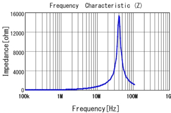
■ LQH32PB100MN0 |Z|
