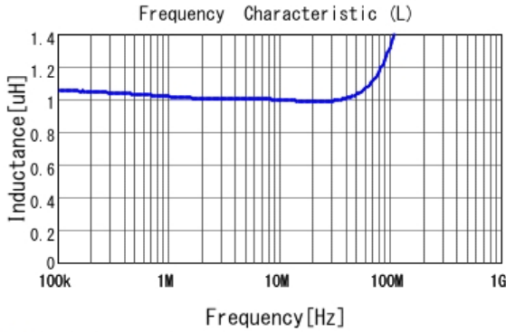
■ LQH43PN1R0N26 L
