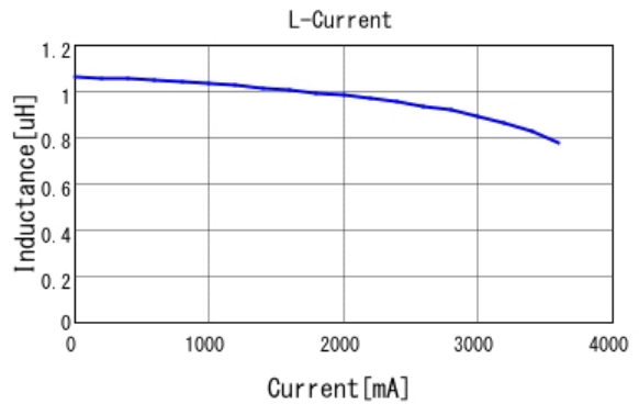
■ LQH43PN1R0N26 L-Current 20degC
