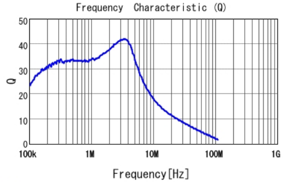
■ LQH43PN1R0N26 Q
