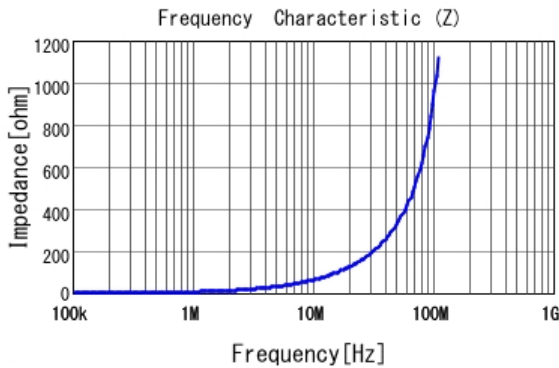
■ LQH43PN1R0N26 |Z|
