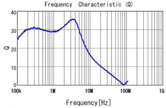
LQH43PN2R2M26 Q
