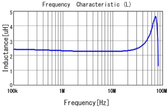
LQH43PN2R2M26 L
