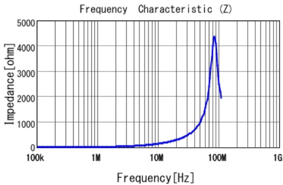
LQH43PN2R2M26 |Z|
