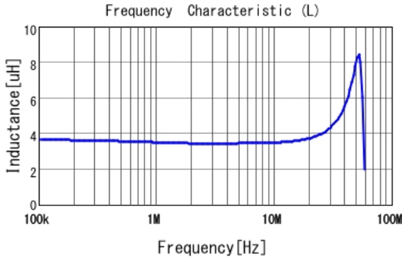
■ LQH43PN3R3M26 L
