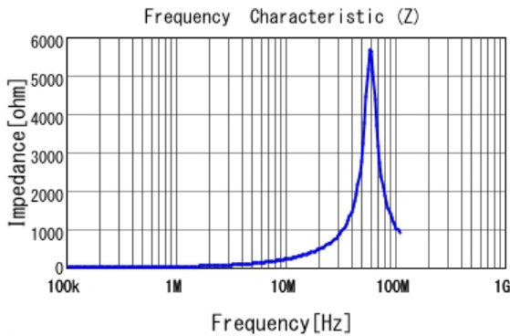
■ LQH43PN3R3M26 |Z|
