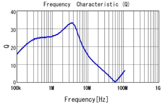
■ LQH43PN3R3M26 Q
