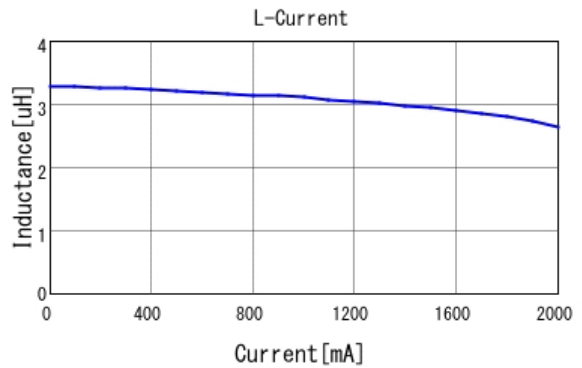
■ LQH43PN3R3M26 L-Current 20degC
