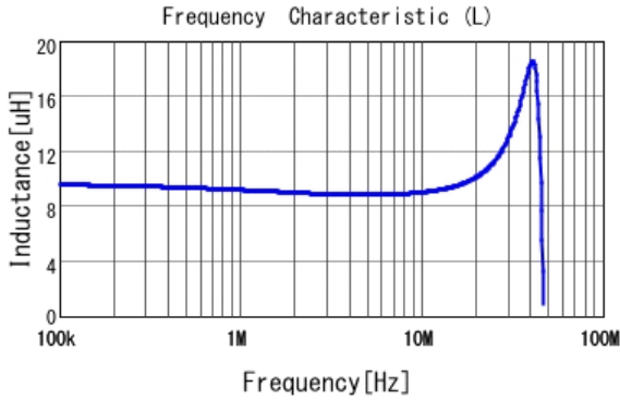
■ LQH44PN100MJ0 L
