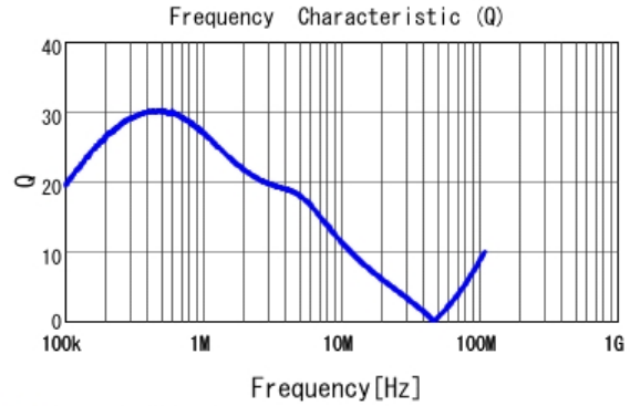
■ LQH44PN100MJ0 Q
