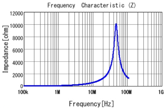
■ LQH44PN100MJ0 |Z|
