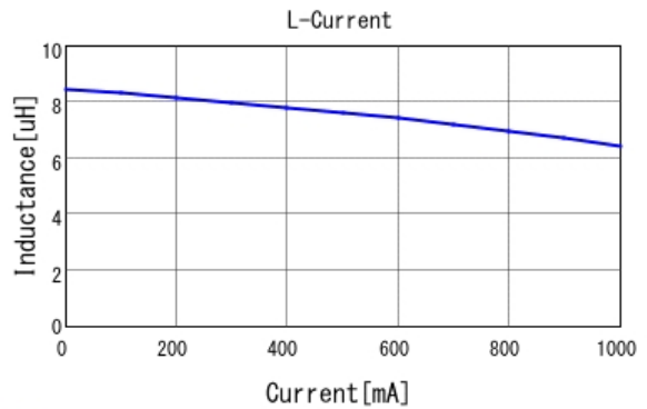
■ LQH44PN100MJ0 L-Current 20degC
