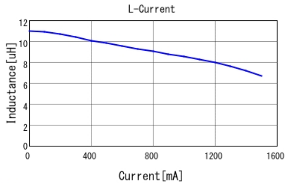
■ LQH44PN100MP0 L-Current 20degC
