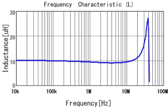
■ LQH44PN100MP0 L
