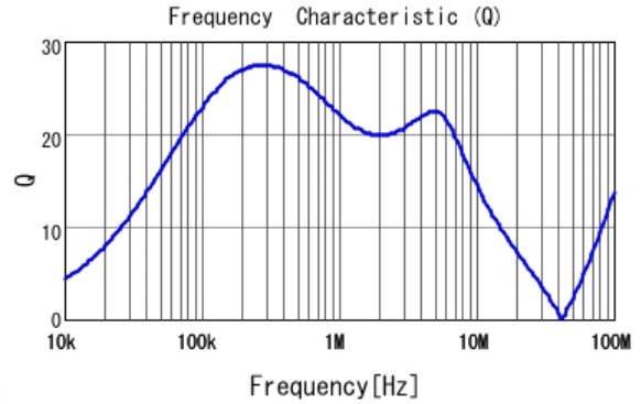
■ LQH44PN100MP0 Q
