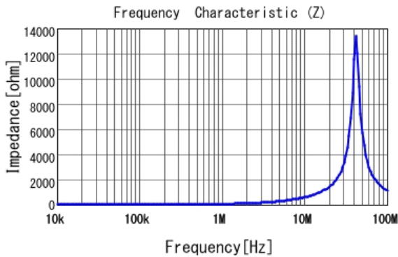
■ LQH44PN100MP0 |Z|
