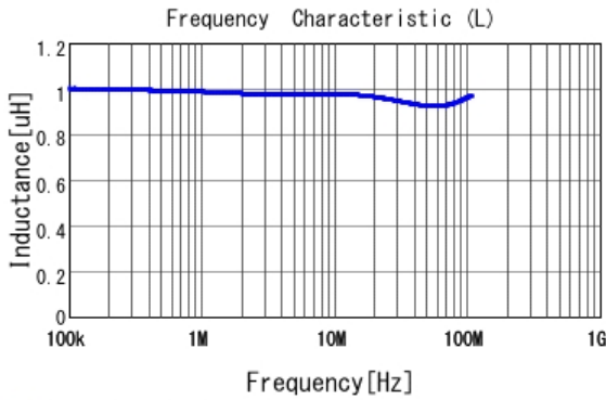
■ LQH44PN1R0NJ0 L
