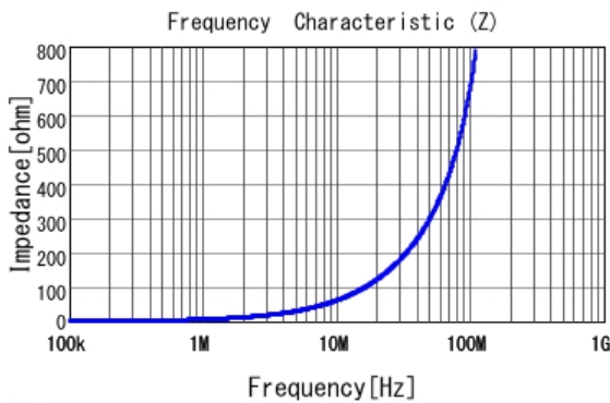
■ LQH44PN1R0NJ0 |Z|
