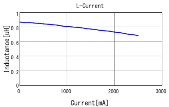
■ LQH44PN1R0NJ0 L-Current 20degC
