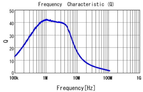
■ LQH44PN1R0NJ0 Q
