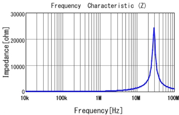
LQH44PN220MP0 |Z|
