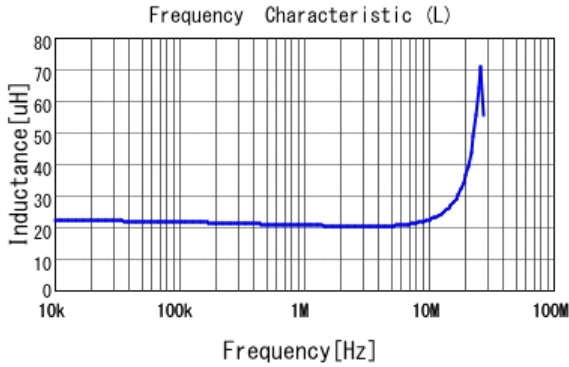
LQH44PN220MP0 L
