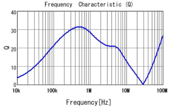
LQH44PN220MP0 Q
