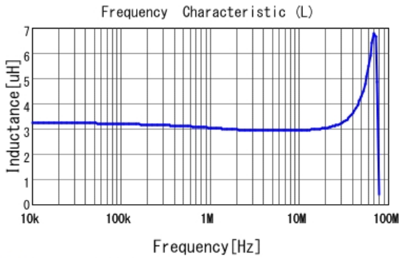
■ LQH44PN3R3MP0 L
