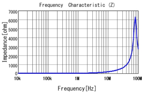
■ LQH44PN3R3MP0 |Z|
