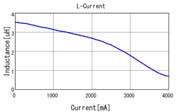
■ LQH44PN3R3MP0 L-Current 20degC
