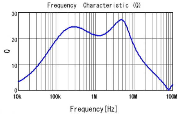
■ LQH44PN3R3MP0 Q
