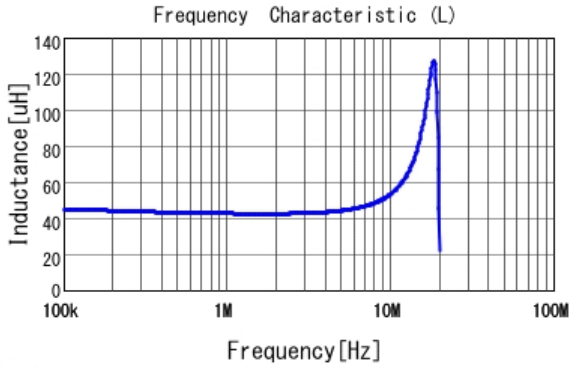
■ LQH44PN470MJ0 L
