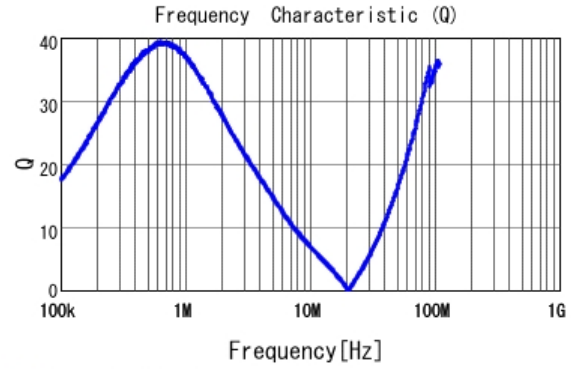
■ LQH44PN470MJ0 Q
