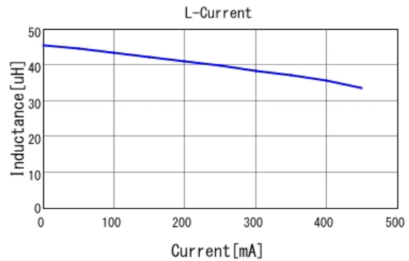
■ LQH44PN470MJ0 L-Current 20degC
