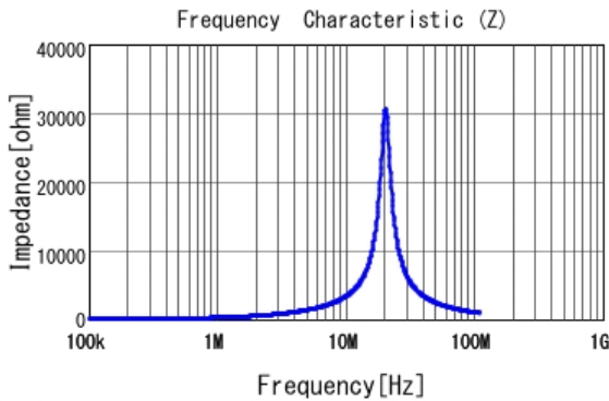
■ LQH44PN470MJ0 |Z|
