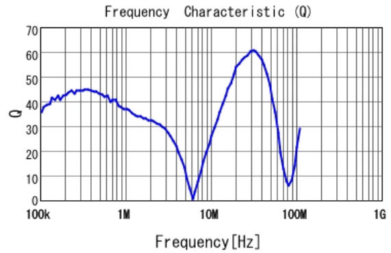
■ LQH5BPN101M38 Q
