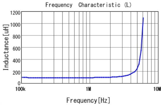
■ LQH5BPN101M38 L
