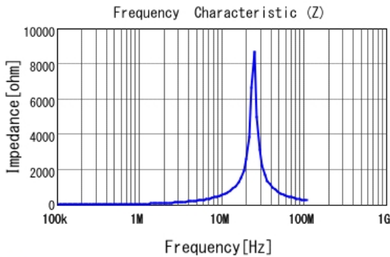
■ LQH5BPN6R8M38 |Z|
