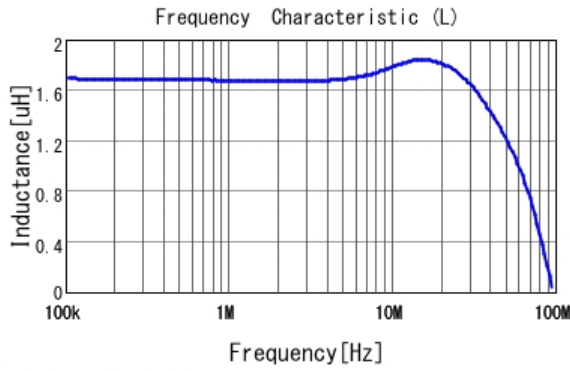
■ LQM18PN1R5NB0 L
