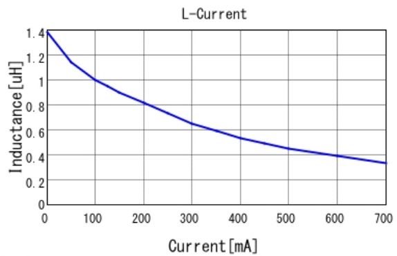
■ LQM18PN1R5NB0 L-Current 20degC
