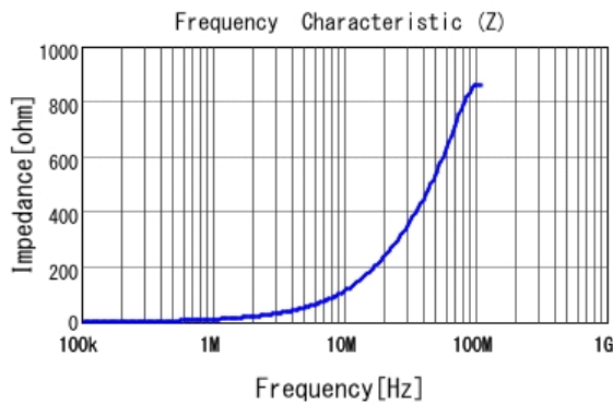
■ LQM18PN1R5NB0 |Z|
