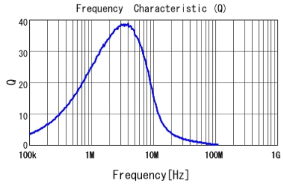
■ LQM18PN1R5NB0 Q
