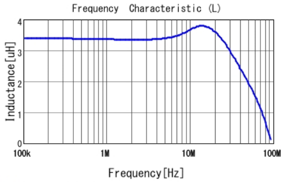
■ LQM18PN3R3MFR L
