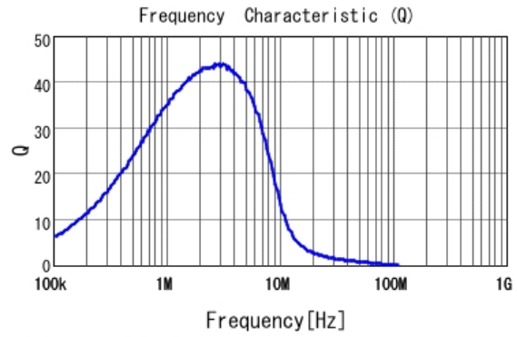
■ LQM18PN3R3MFR Q
