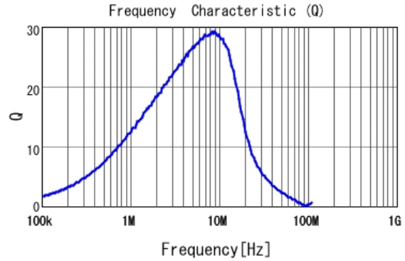
■ LQM21PN1R0MEH Q
