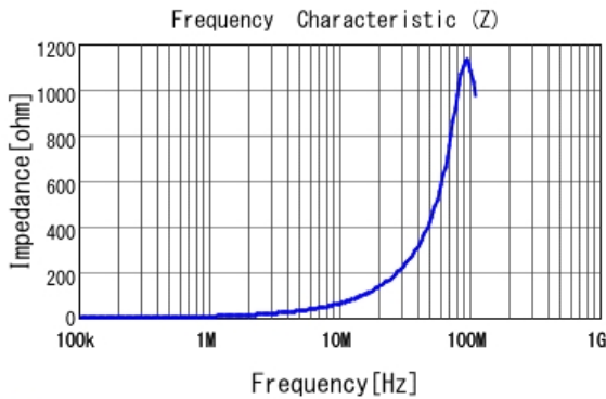
■ LQM21PN1R0MEH |Z|
