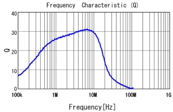
■ LQM21PN1R0NGC Q
