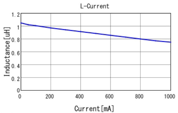
■ LQM21PN1R0NGC L-Current 20degC
