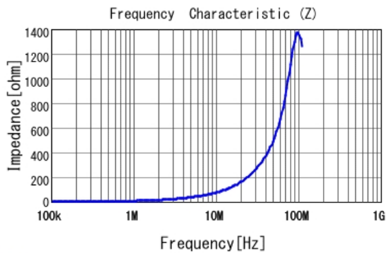
■ LQM21PN1R0NGC |Z|
