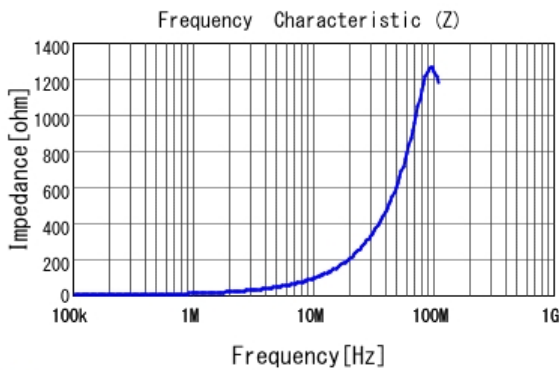
■ LQM21PN1R5MC0 |Z|
