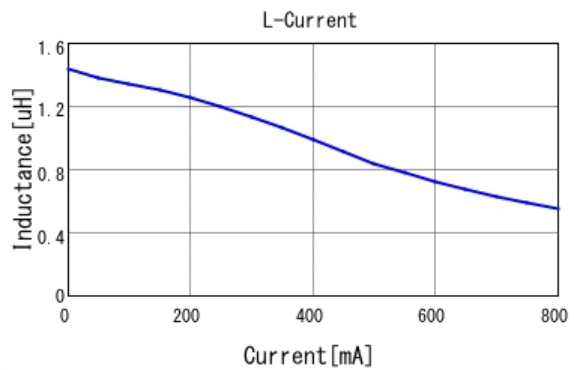
■ LQM21PN1R5MC0 L-Current 20degC
