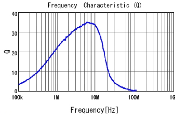
■ LQM21PN1R5MC0 Q
