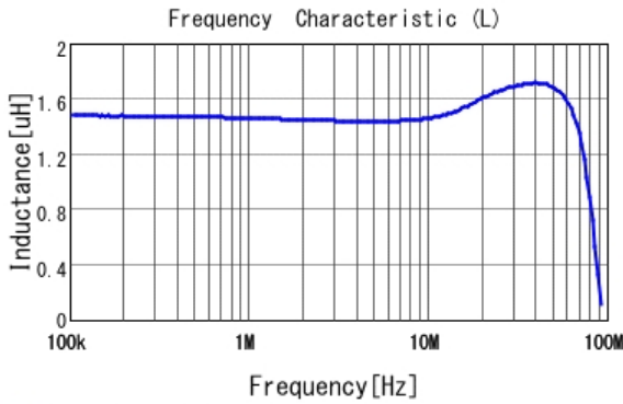
■ LQM21PN1R5MC0 L
