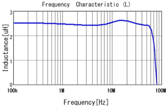
■ LQM21PN2R2NGC L
