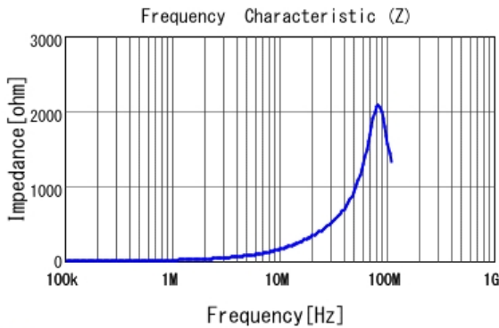
■ LQM21PN2R2NGC |Z|
