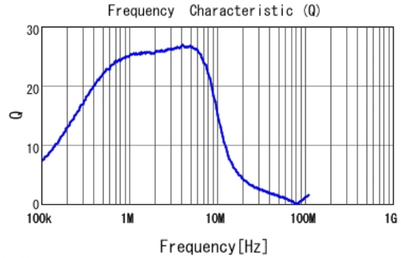
■ LQM21PN2R2NGC Q
