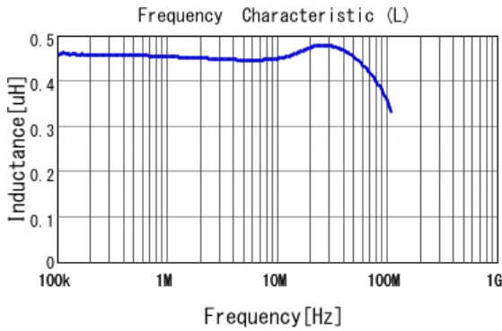
■ LQM21PZR47MC0 L
