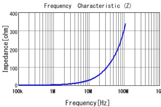
■ LQM21PZR47MC0 |Z|
