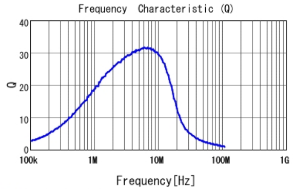
■ LQM21PZR47MC0 Q
