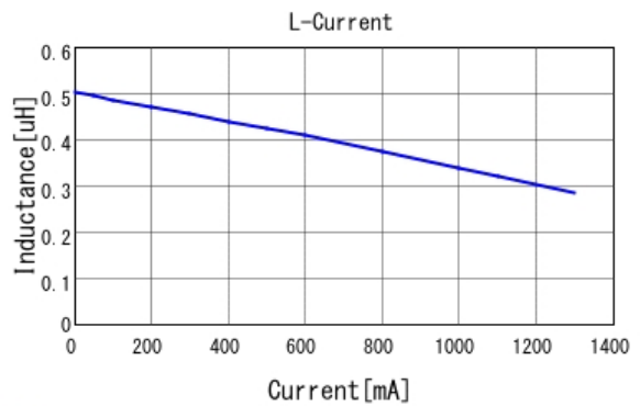
■ LQM21PZR47MC0 L-Current 20degC
