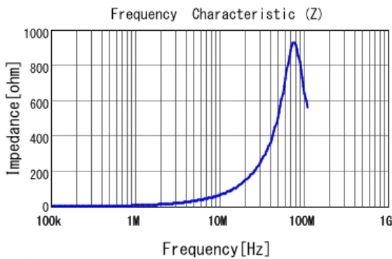
LQM2HPN1R0MG0 |Z|
