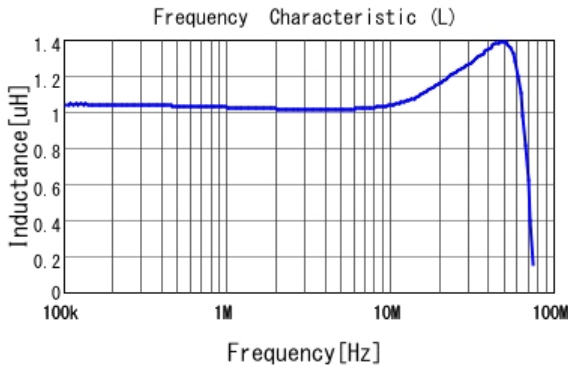
LQM2HPN1R0MG0 L
