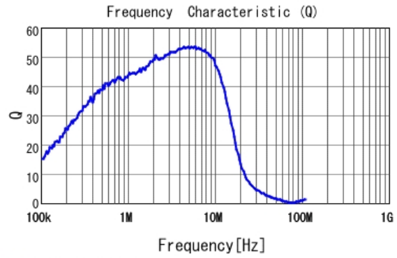
LQM2HPN1R0MG0 Q
