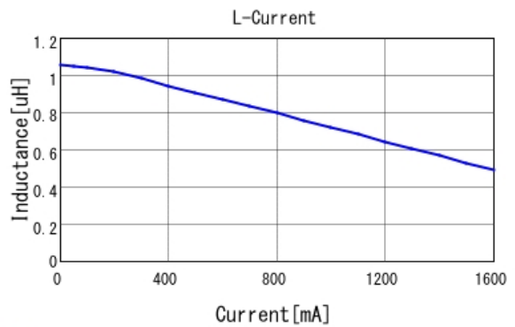
LQM2HPN1R0MG0 L-Current 20degC
