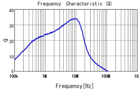
■ LQM2HPN1R0MJ0 Q
