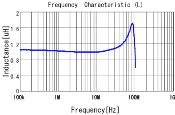
■ LQM2HPN1R0MJ0 L
