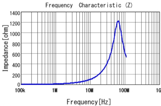
■ LQM2HPN1R5MG0 |Z|
