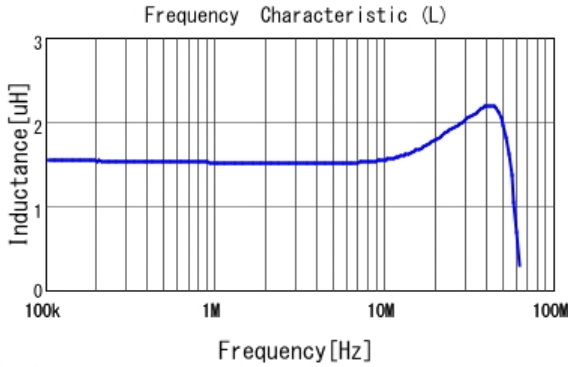
■ LQM2HPN1R5MG0 L
