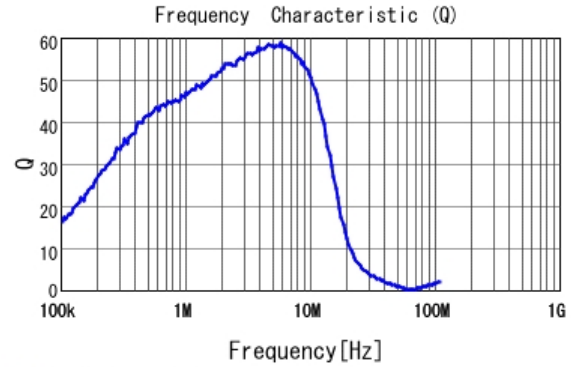
■ LQM2HPN1R5MG0 Q
