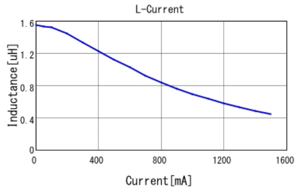
■ LQM2HPN1R5MG0 L-Current 20degC
