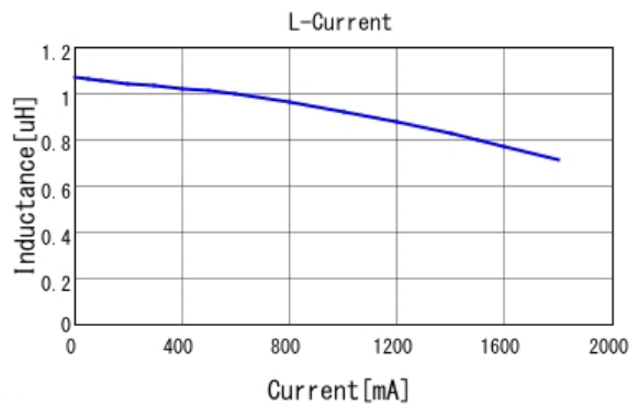
LQM2HPZ1R0MJ0 L-Current 20degC
