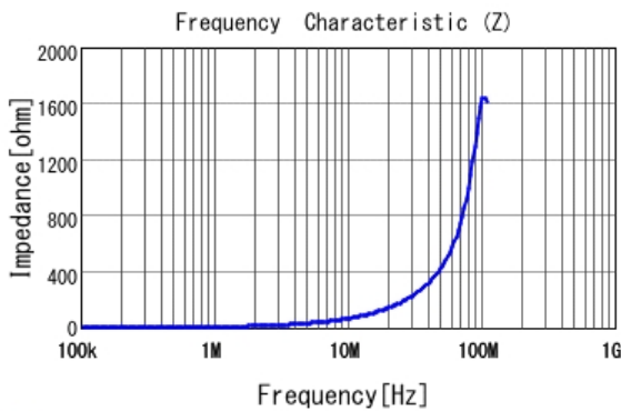
■ LQM2MPN1R0NG0 |Z|
