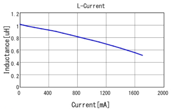
■ LQM2MPN1R0NG0 L-Current 20degC
