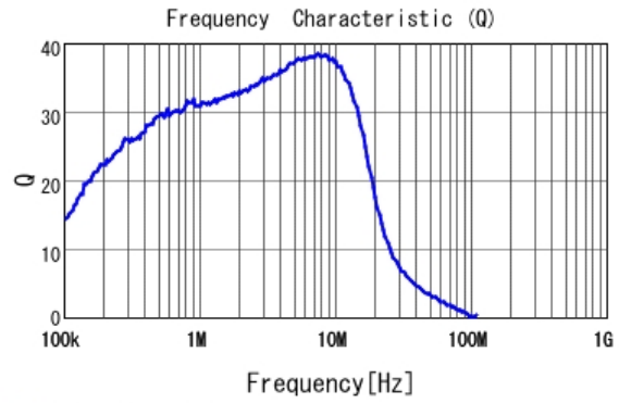
■ LQM2MPN1R0NG0 Q
