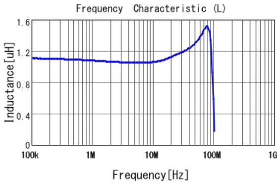
■ LQM2MPN1R0NG0 L
