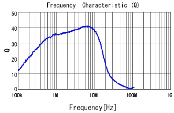
■ LQM2MPN1R5MG0 Q
