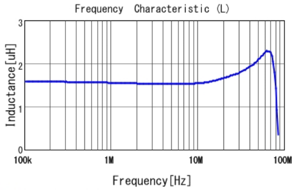
■ LQM2MPN1R5MG0 L
