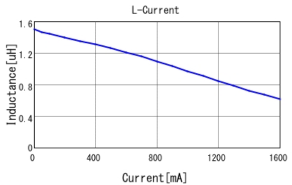
■ LQM2MPN1R5MG0 L-Current 20degC
