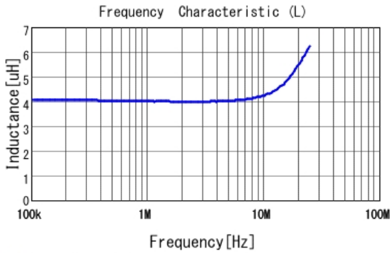
LQM2MPN4R7MG0 L
