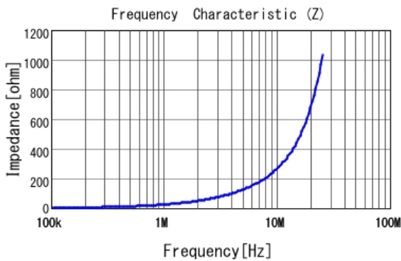
LQM2MPN4R7MG0 |Z|
