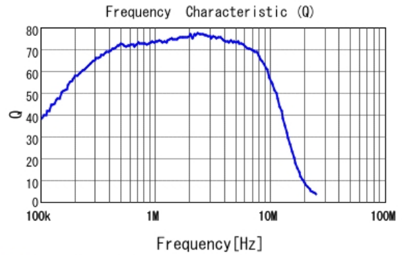
LQM2MPN4R7MG0 Q
