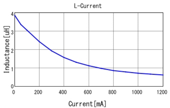
LQM2MPN4R7MG0 L-Current 20degC
