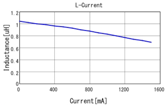
■ LQM31PN1R0M00 L-Current 20degC
