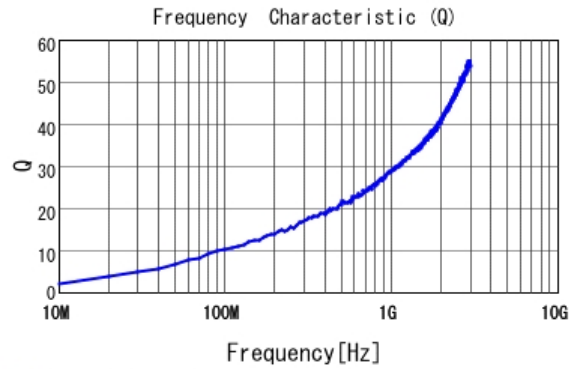
■ LQP02HQ1N0B02 Q
