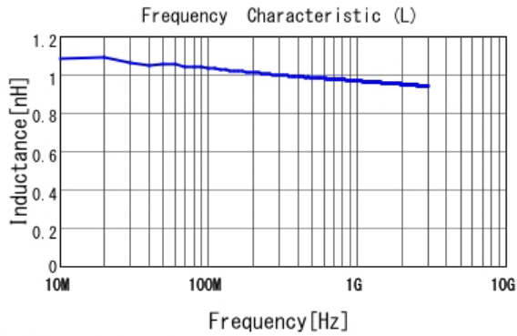
■ LQP02HQ1N0B02 L
