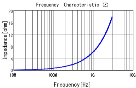
■ LQP02HQ1N0B02 |Z|
