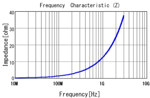
■ LQP02HQ2N0B02 |Z|
