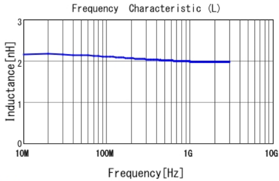
■ LQP02HQ2N0B02 L
