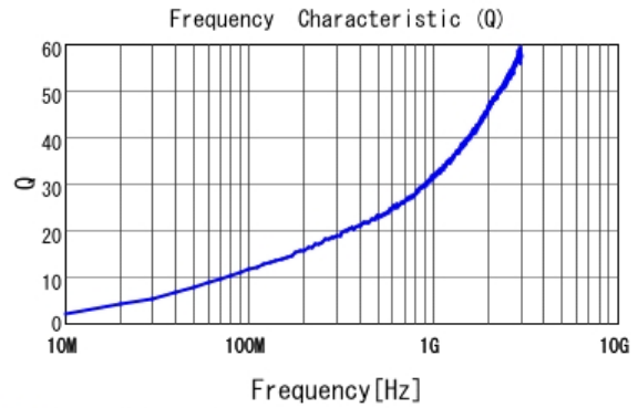
■ LQP02HQ2N0B02 Q
